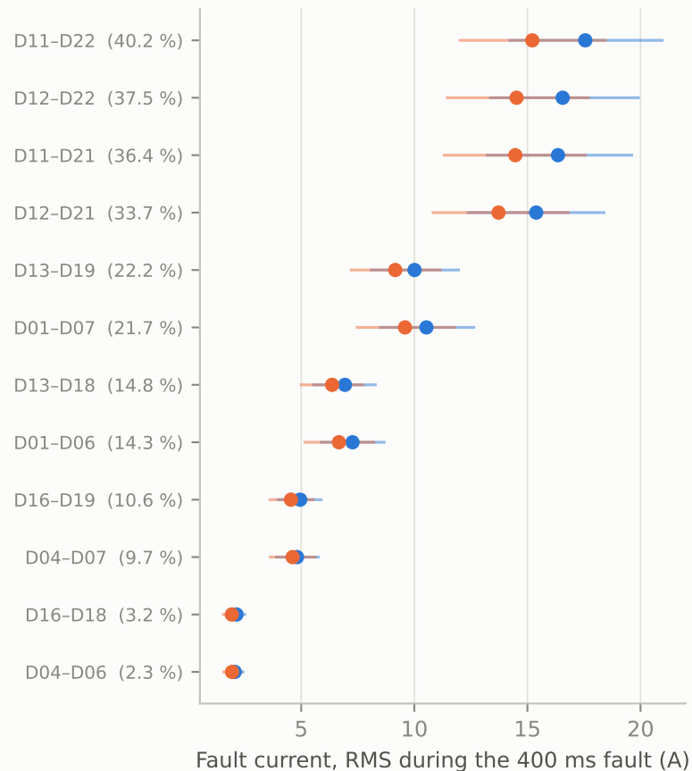
Inter-winding short-circuits
