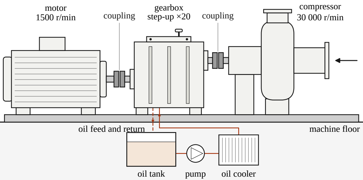
(a) Geared train
