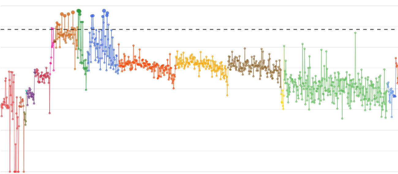
DNa15: flight
