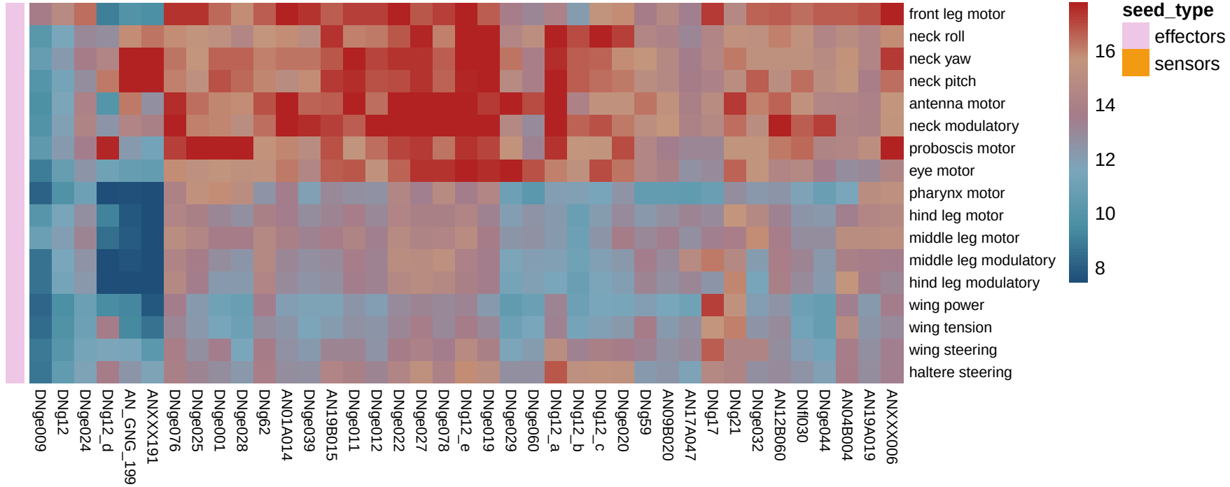
influence_norm_log (row: target, col: source)
