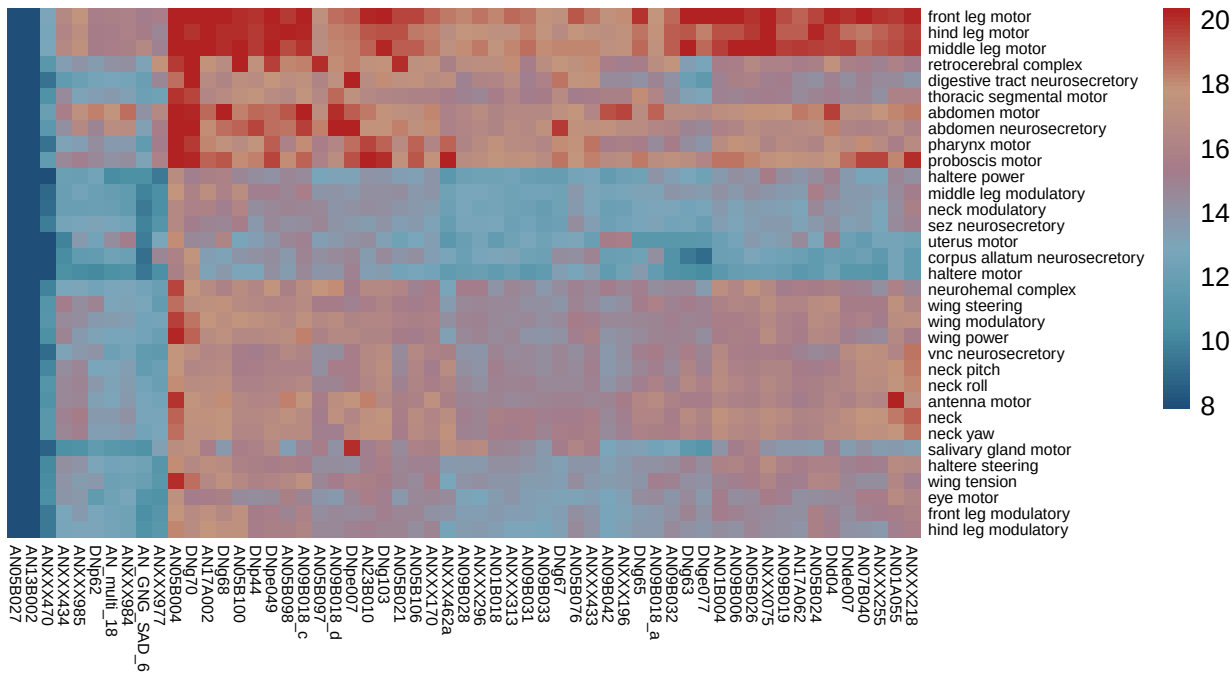
full influence_norm_log (rows: effectors, cols: AN/DN cell types)
