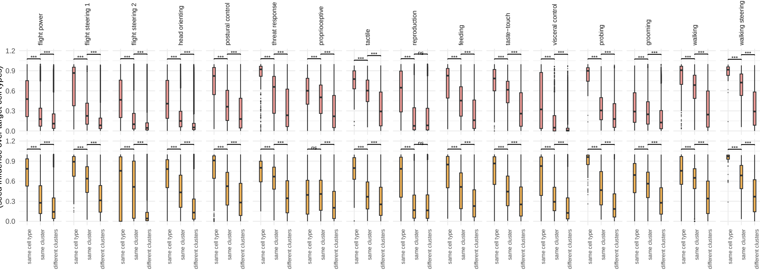
cosine similarity
