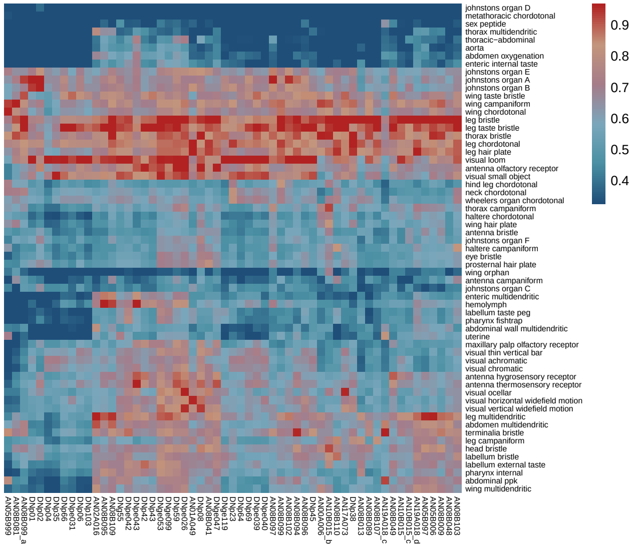
full influence_log_minmax (rows: sensors, cols: AN/DN cell types)
