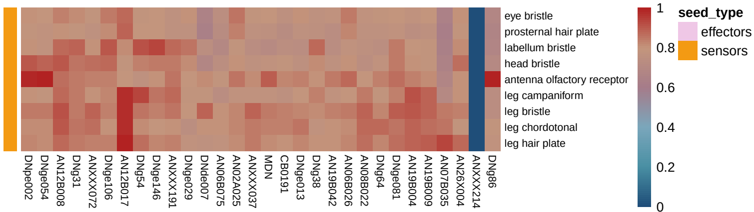
influence_log_rownorm (row: source, col: target)
