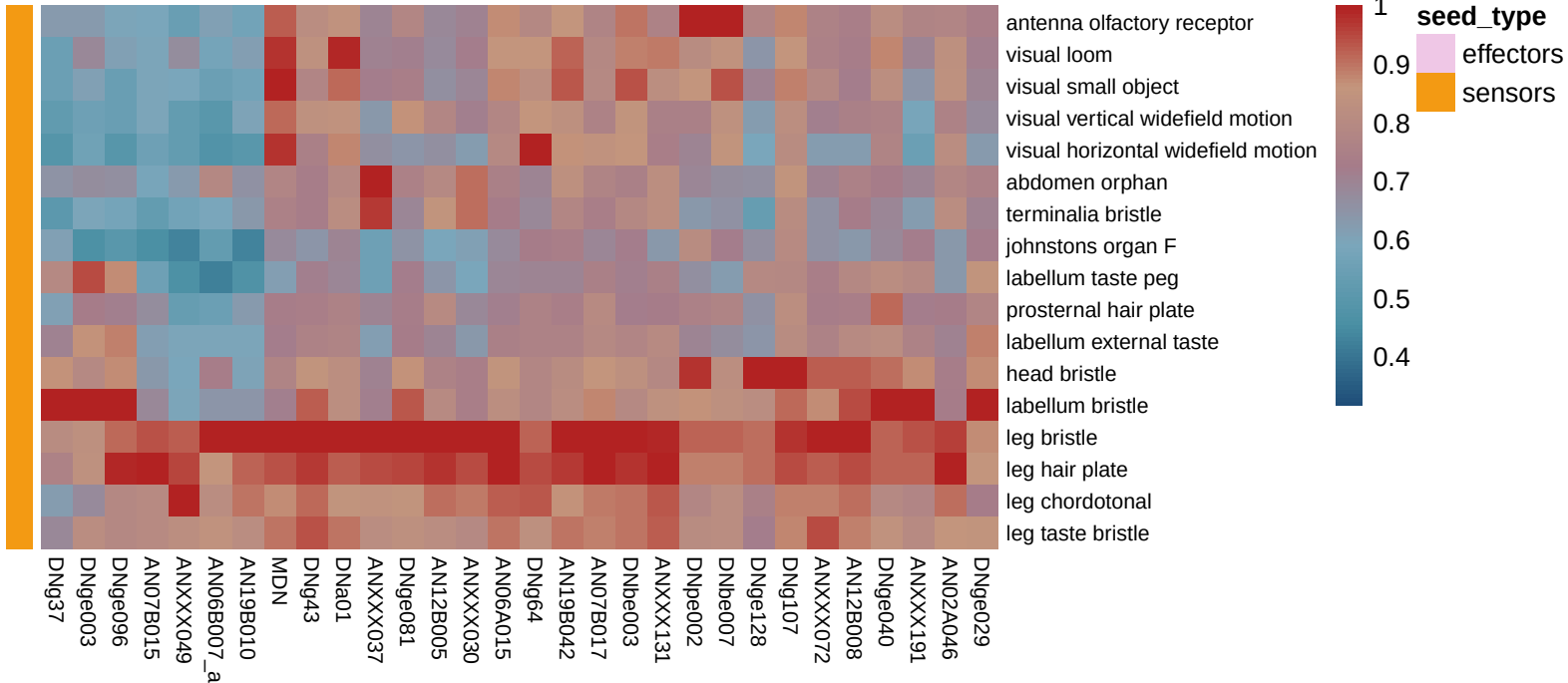
influence_log_minmax (row: source, col: target)
