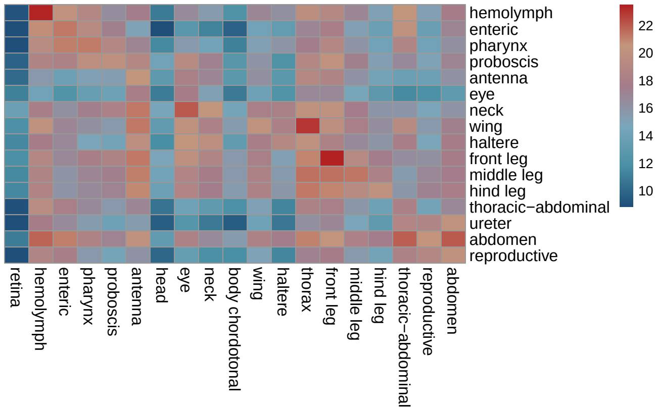
influence_norm_log
