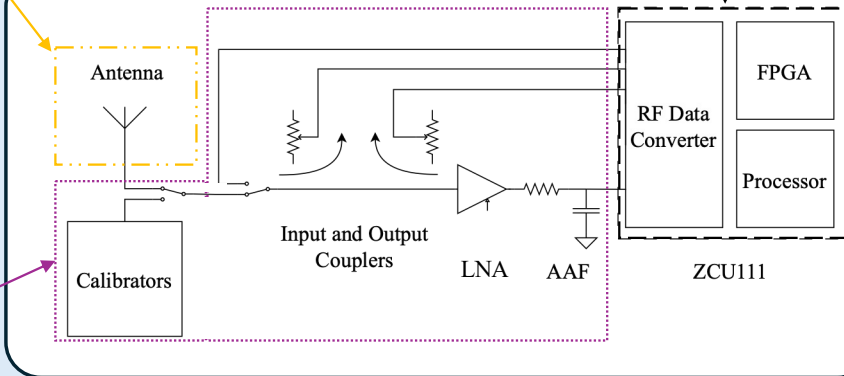
CosmoCube payload diagram
