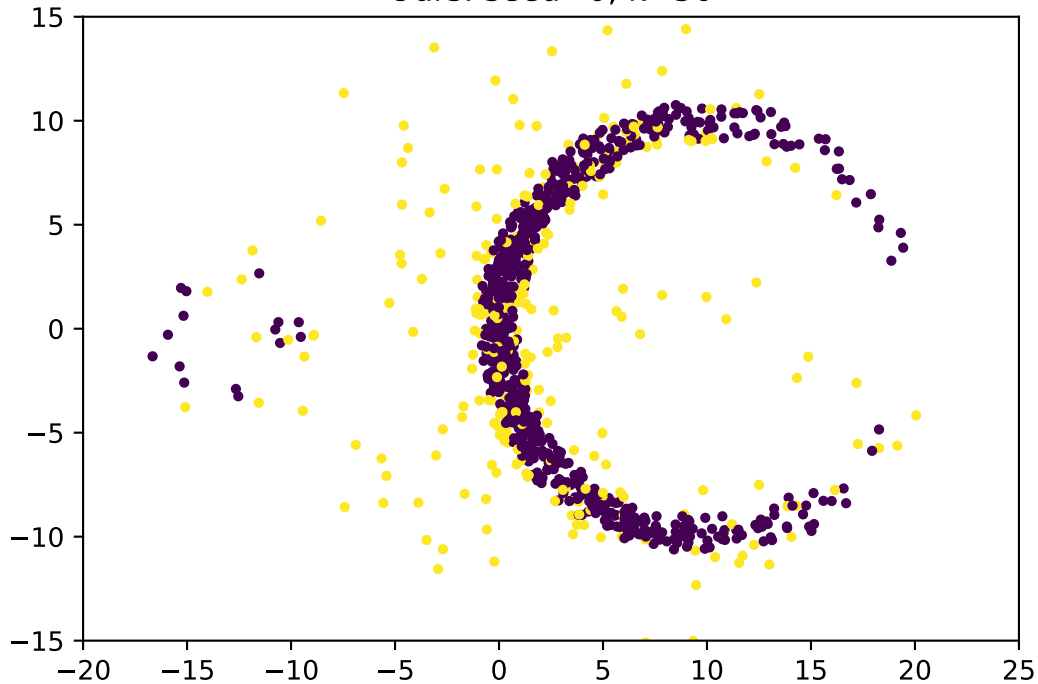
Ours: seed=0, k=50
