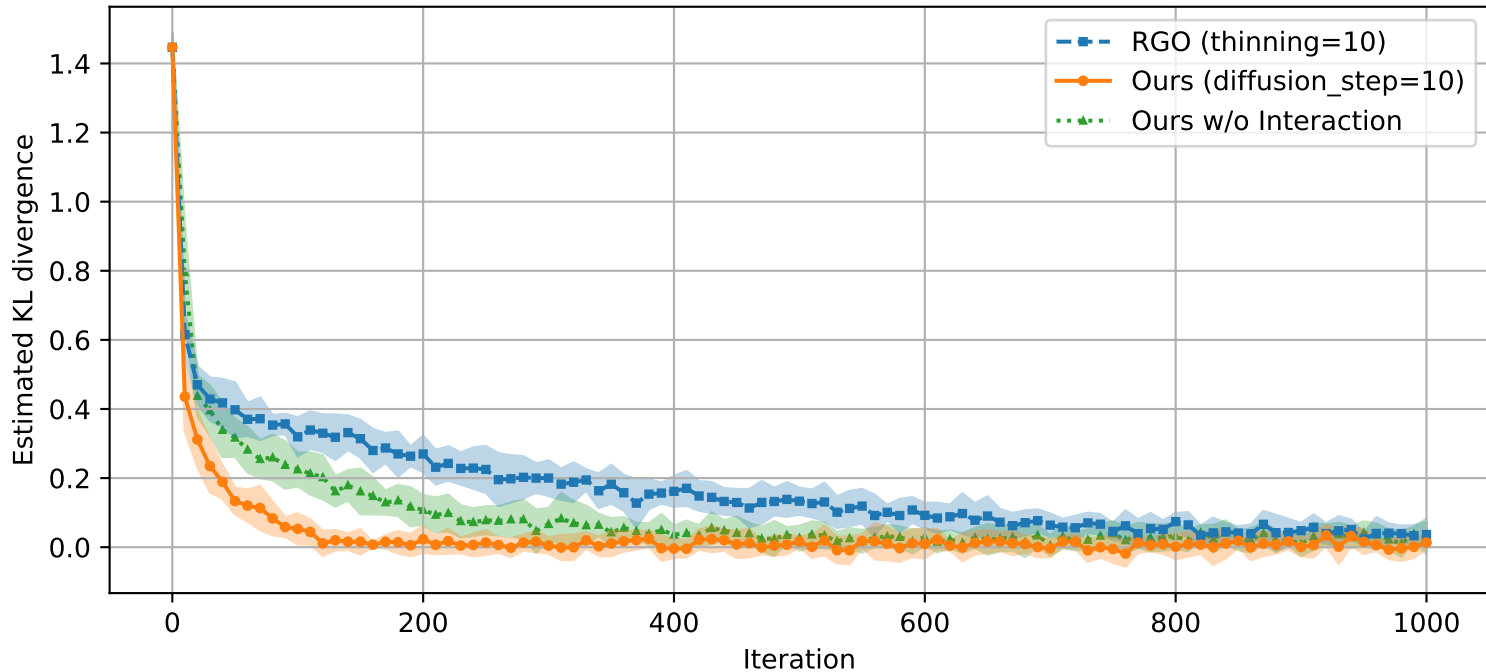
KL divergence (100 particles vs 100 chains, aggregated every 10 steps)
