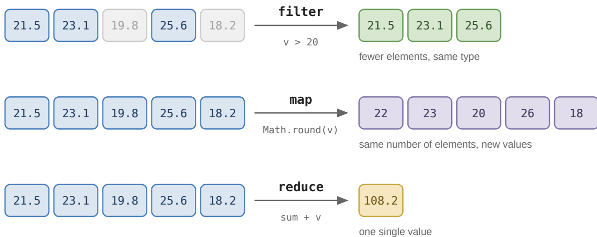
Figure 2.2.1: filter keeps some elements, map turns every element into a new one, reduce produces a single value
