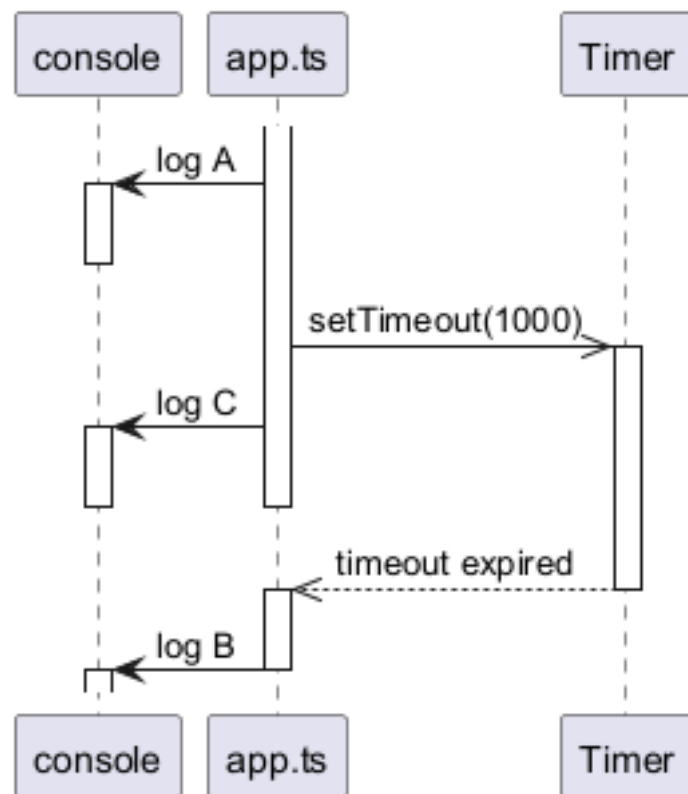
Figure 2.3.1: sequence diagram: app.ts logs A, hands the timer a callback, logs C, and only when the timer has expired does the callback log B
