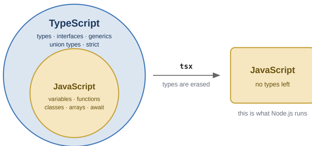
Figure 2.1.1: JavaScript sits inside TypeScript: TypeScript adds types, interfaces, generics, union types and strict mode, and after tsx has run only plain JavaScript is left
