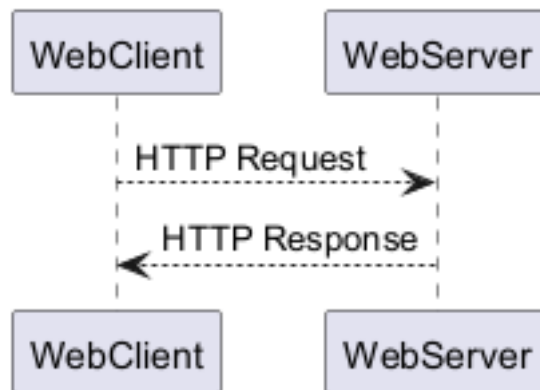
Figure 2.4.1: sequence diagram: a web client sends an HTTP request to a web server, which sends back an HTTP response
