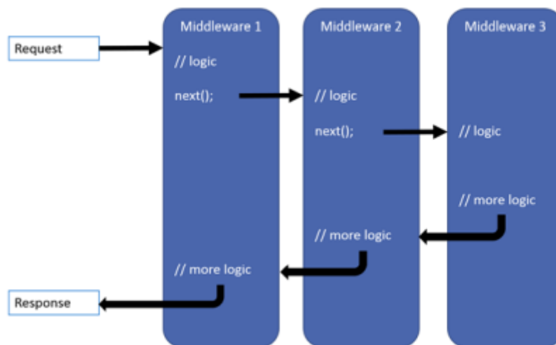
Figure 2.4.2: the request passes through middleware 1, 2 and 3, each running some logic and calling next() , and the response travels back out through the same chain in reverse
