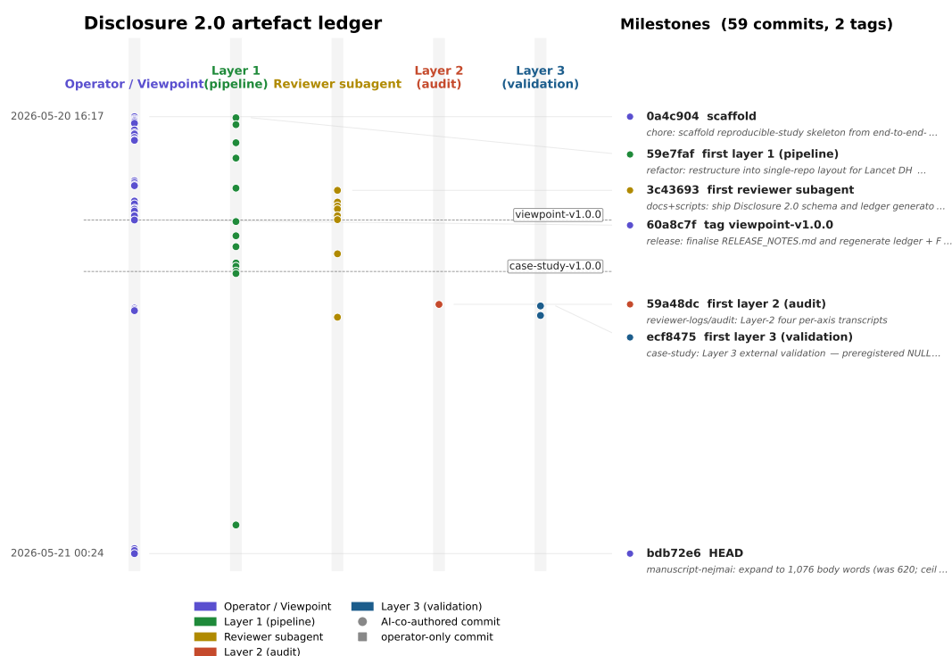
Figure 1: Disclosure 2.0 artefact ledger for the supporting case study, regenerated from git log on each release tag. Markers: commits coloured by AI-co-authorship status, reviewer-subagent rounds, audit checkpoints, and tagged release.
