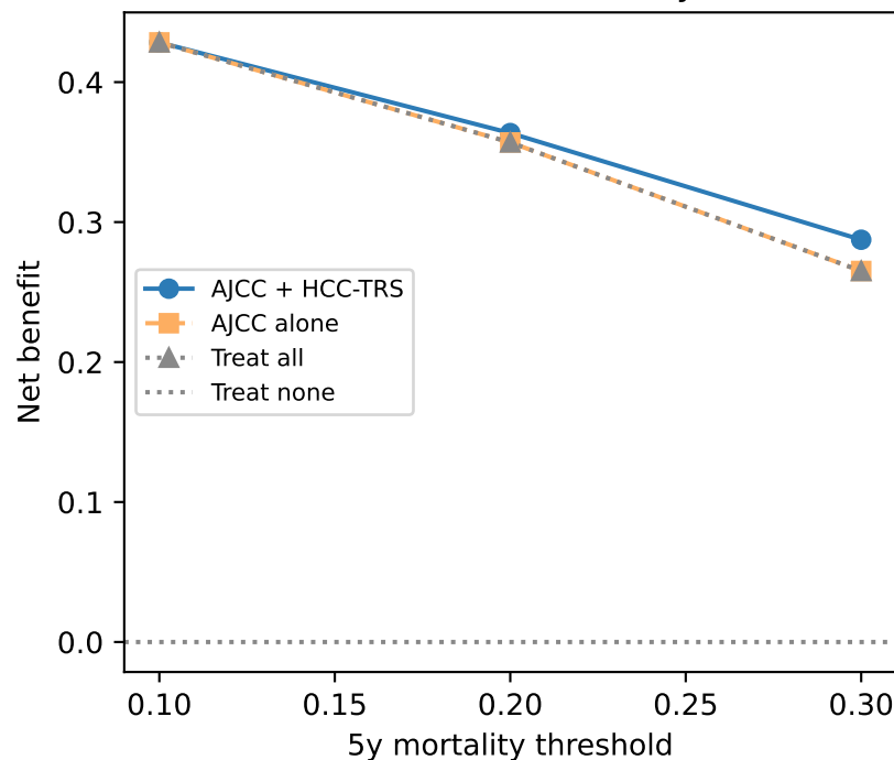
Decision-curve at 5 y
