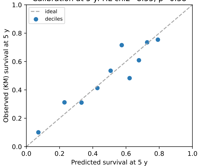
Calibration at 5 y: HL \chi^2=8.55 , p=0.38
