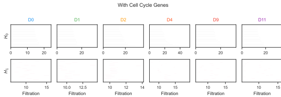
(c) Barcodes with cell-cycle genes.
