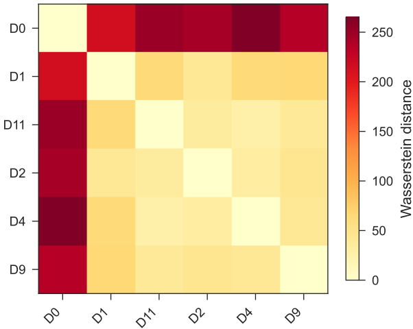
H Diagram Distances
