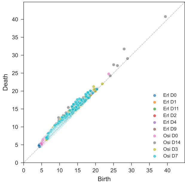
H_1 Persistence Diagram
