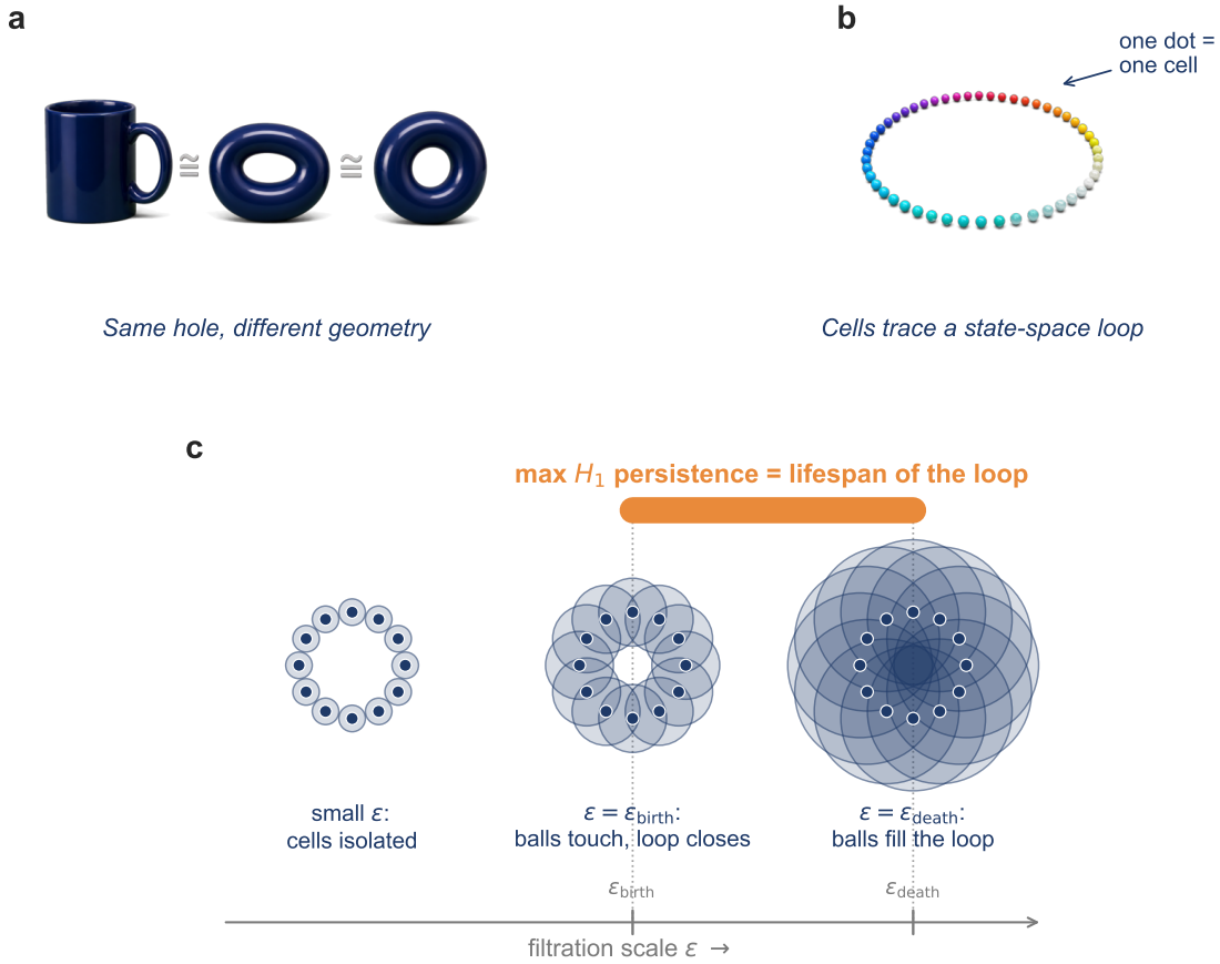
Figure 1: Topology distinguishes shapes that geometry cannot. (a) Mug and donut share one hole and are continuously deformable into one another — topologically equivalent despite different geometry. (b) Cells reversibly cycling among states lie on a closed loop in state-space; the loop itself is the invariant. (c) Persistent homology summarises this as a barcode: short bars reflect noise ( H_0 components); one long H_1 bar (orange) marks a robust loop. Its lifetime is the maximum H_1 persistence used throughout this work.
