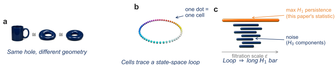
Figure 1: Topology distinguishes shapes that geometry cannot. (a) Mug and donut share one hole and are continuously deformable into one another — topologically equivalent despite different geometry. (b) Cells reversibly cycling among states lie on a closed loop in state-space; the loop itself is the invariant. (c) Persistent homology summarises this as a barcode: short bars reflect noise ( H_0 components); one long H_1 bar (orange) marks a robust loop. Its lifetime is the maximum H_1 persistence used throughout this work.
