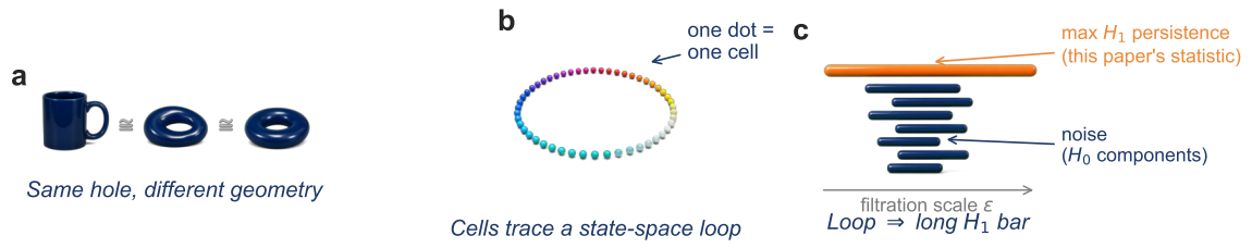
Figure 1: Topology distinguishes shapes that geometry cannot. (a) Mug and donut share one hole and are continuously deformable into one another — topologically equivalent despite different geometry. (b) Cells reversibly cycling among states lie on a closed loop in state-space; the loop itself is the invariant. (c) Persistent homology summarises this as a barcode: short bars reflect noise ( H_0 components); one long H_1 bar (orange) marks a robust loop. Its lifetime is the maximum H_1 persistence used throughout this work.
