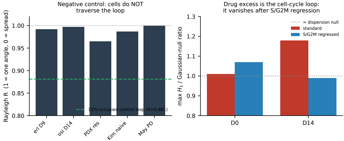
Figure 2: (a) Traversal test: R \geq 0.965 in all cohorts vs 0.881 for a 12%-occupied control. (b) The in-vitro drug excess vanishes after S/G2M regression.
