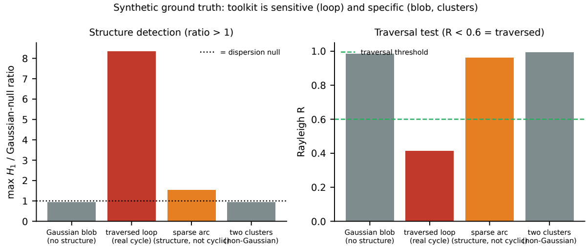
Figure 3: Synthetic ground truth: sensitive (passes the traversed loop) and specific (rejects the Gaussian blob and the two-cluster non-Gaussian case).
