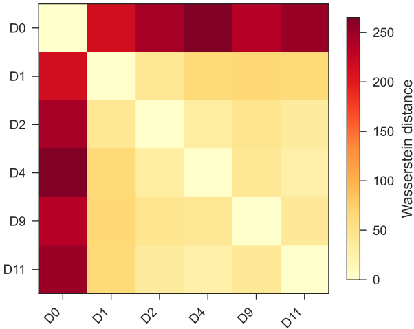
H_1 Diagram Distances
