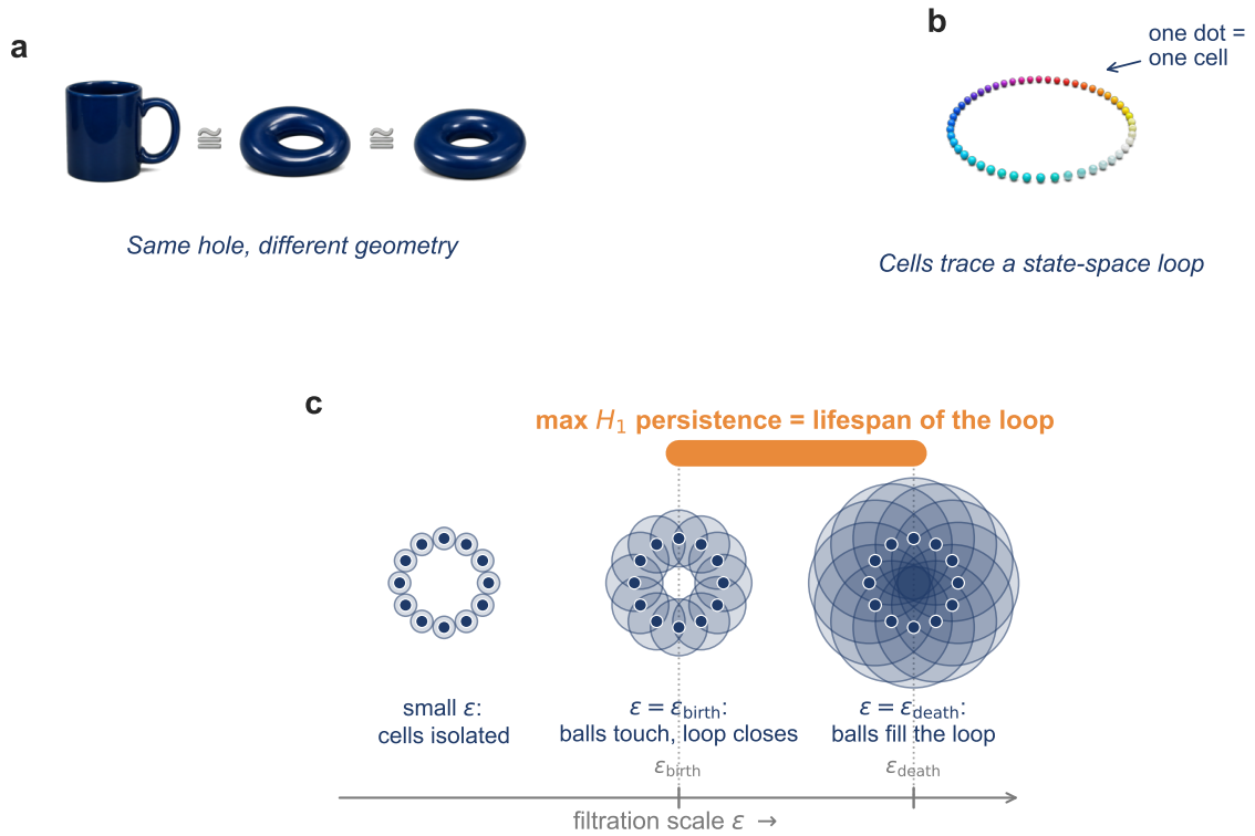
Figure 1: Topology distinguishes shapes that geometry cannot. (a) Mug and donut share one hole and are continuously deformable into one another — topologically equivalent despite different geometry. (b) Cells reversibly cycling among states lie on a closed loop in state-space; the loop itself is the invariant. (c) Persistent homology summarises this as a barcode: short bars reflect noise ( H_0 components); one long H_1 bar (orange) marks a robust loop. Its lifetime is the maximum H_1 persistence used throughout this work.
