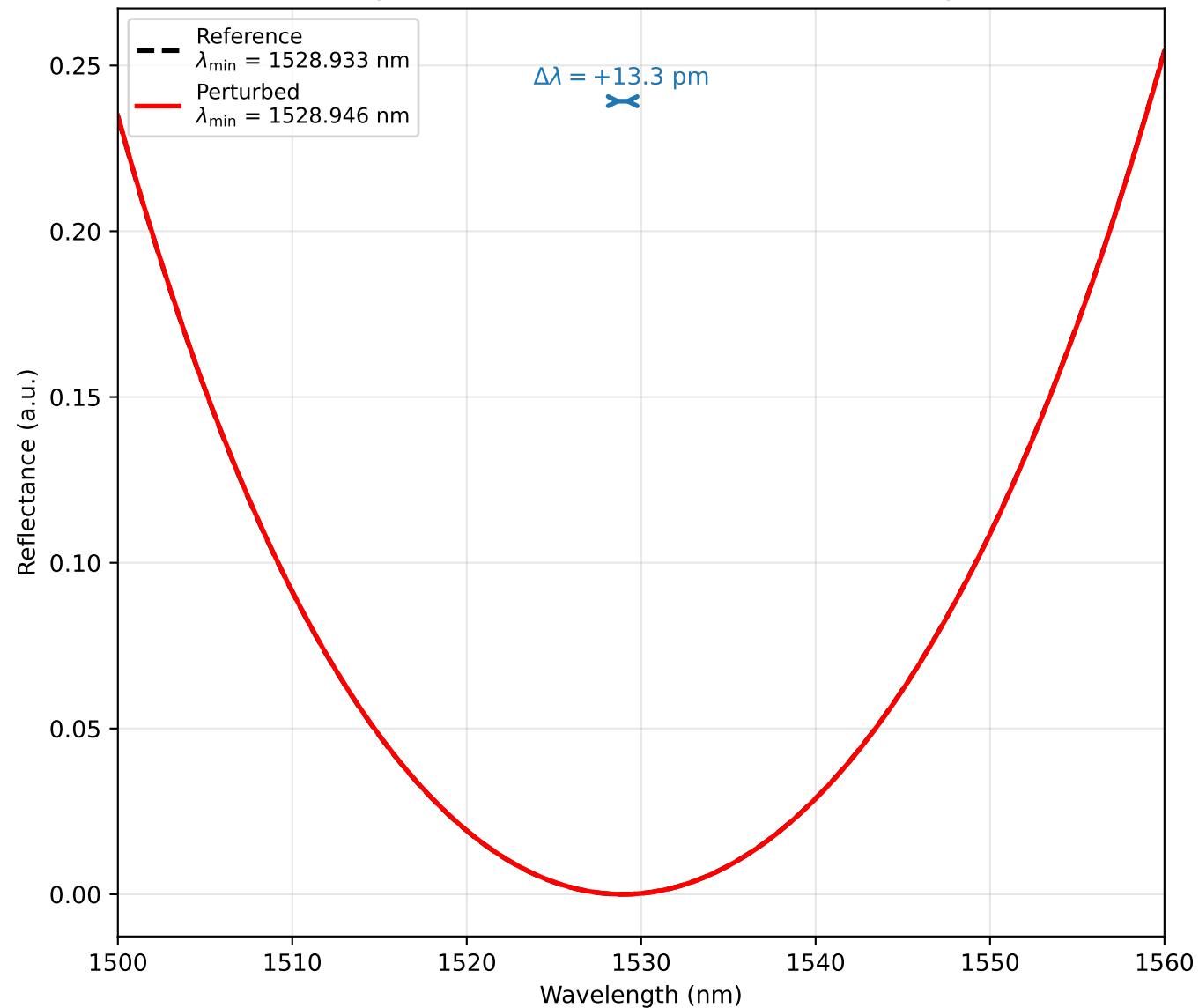
FPI Spectral Shift: Radiation-Induced RI Change
