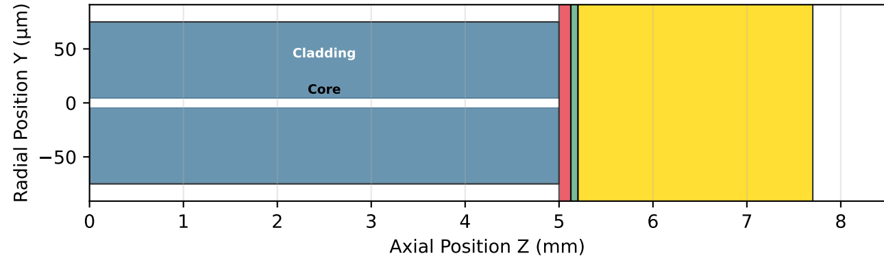
Fiber Sensor Structure (YZ Side View)
