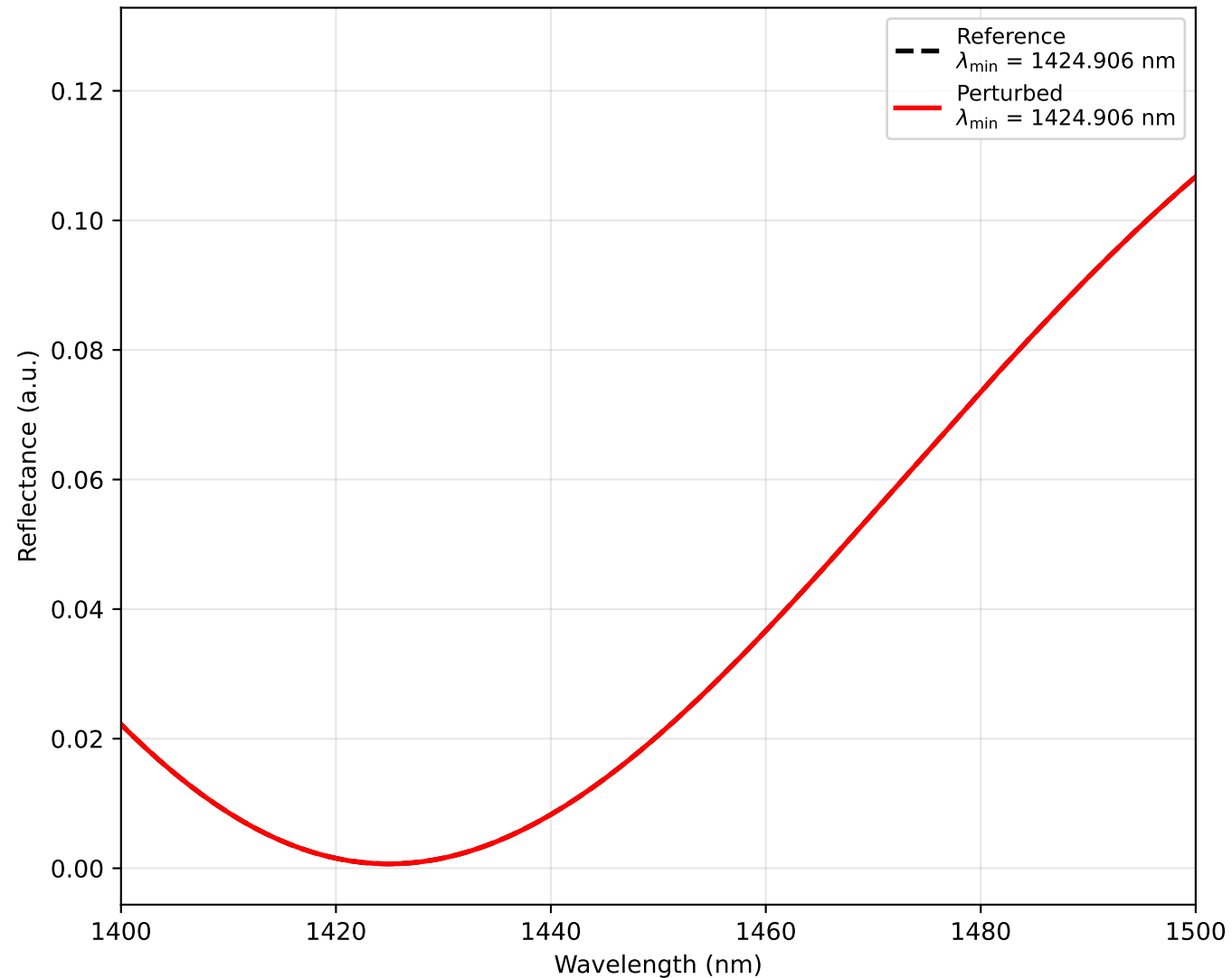
FPI Spectral Shift Due to Radiation Exposure
