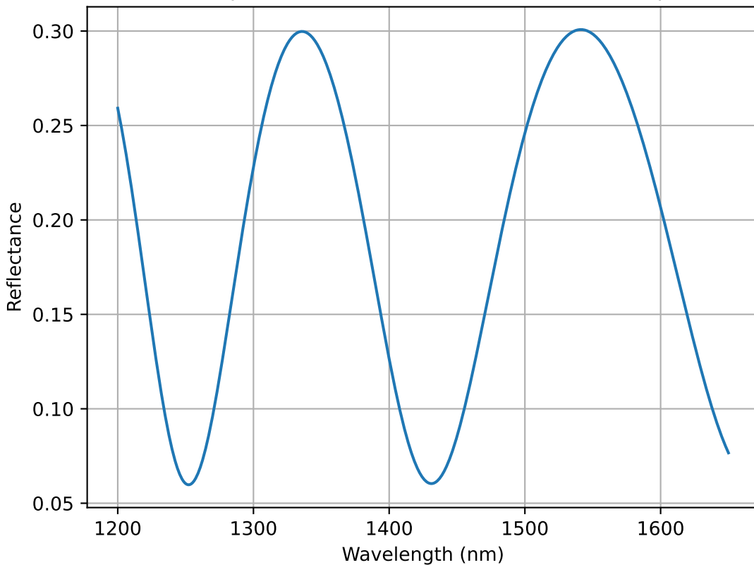
FPI Spectrum - Should Show Resonance Dip
