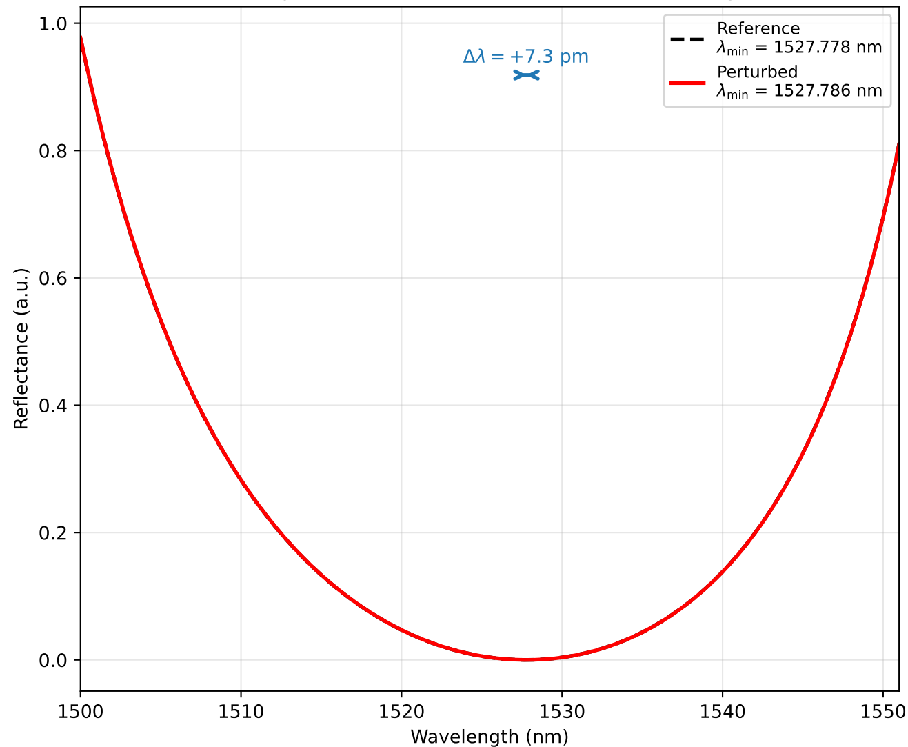
FPI Spectral Shift: Radiation-Induced RI Change
