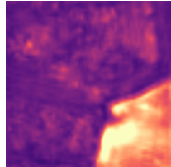
RSCV verified
