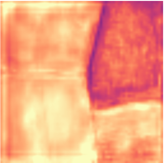
RSCV verified
