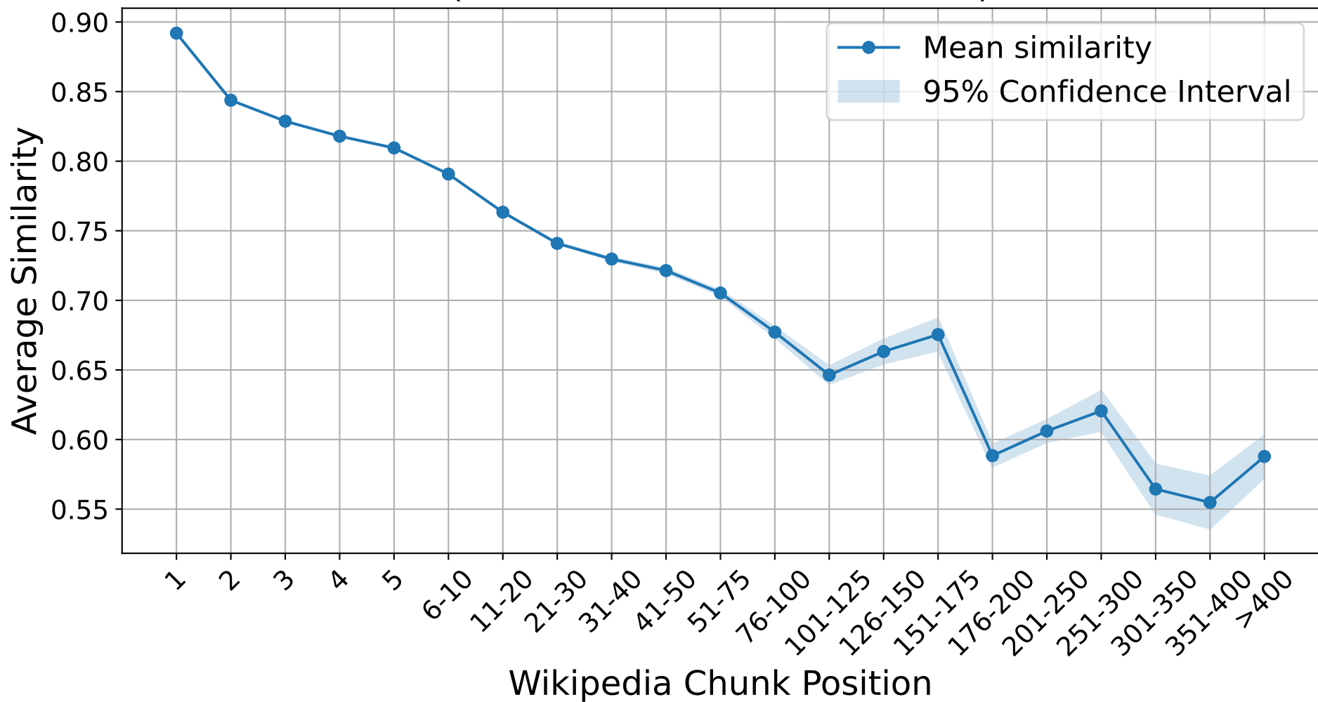
Average Similarity by Wikipedia Chunk Position (with 95% Confidence Intervals)
