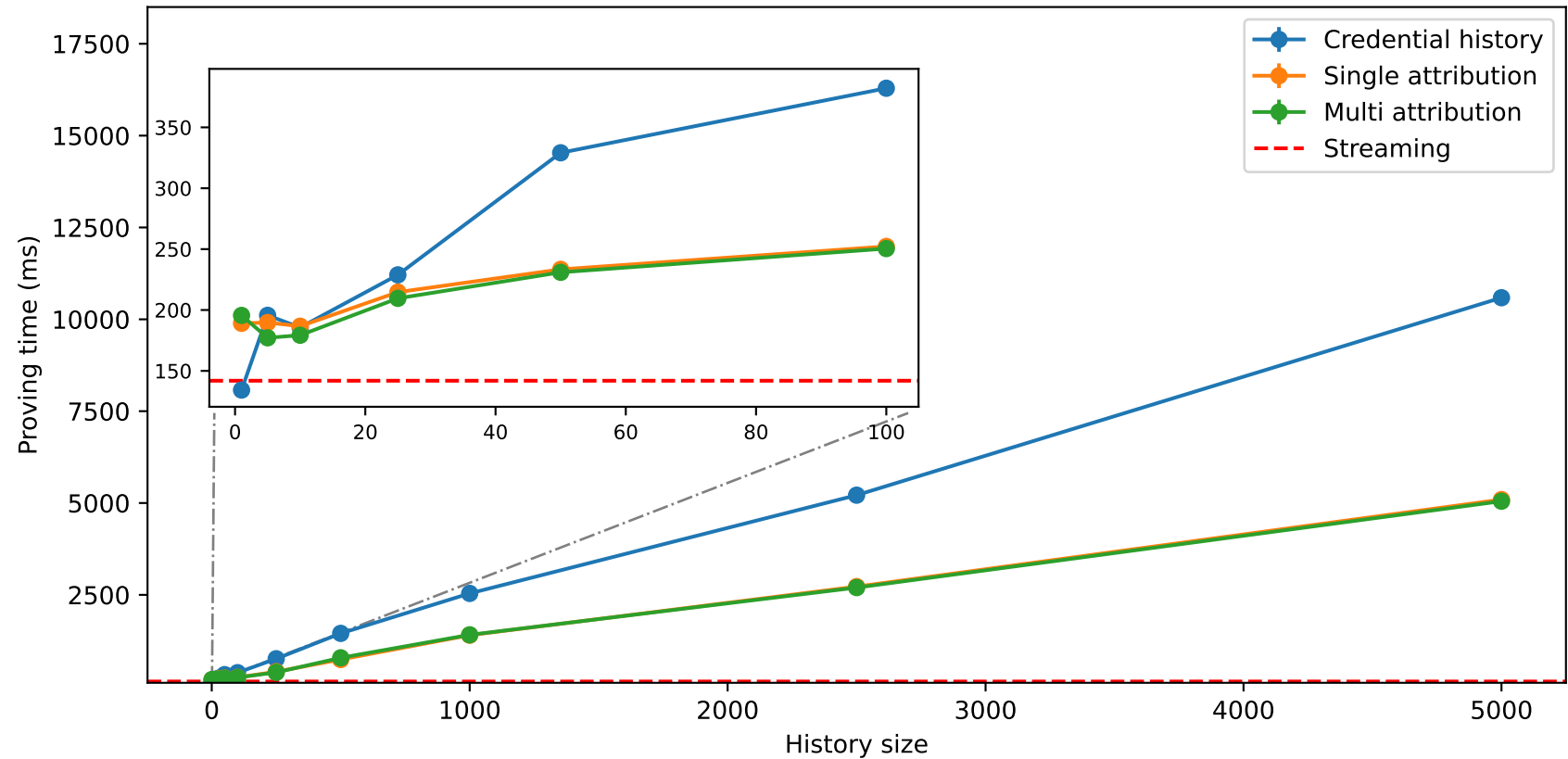
Proving time for all circuit variants
