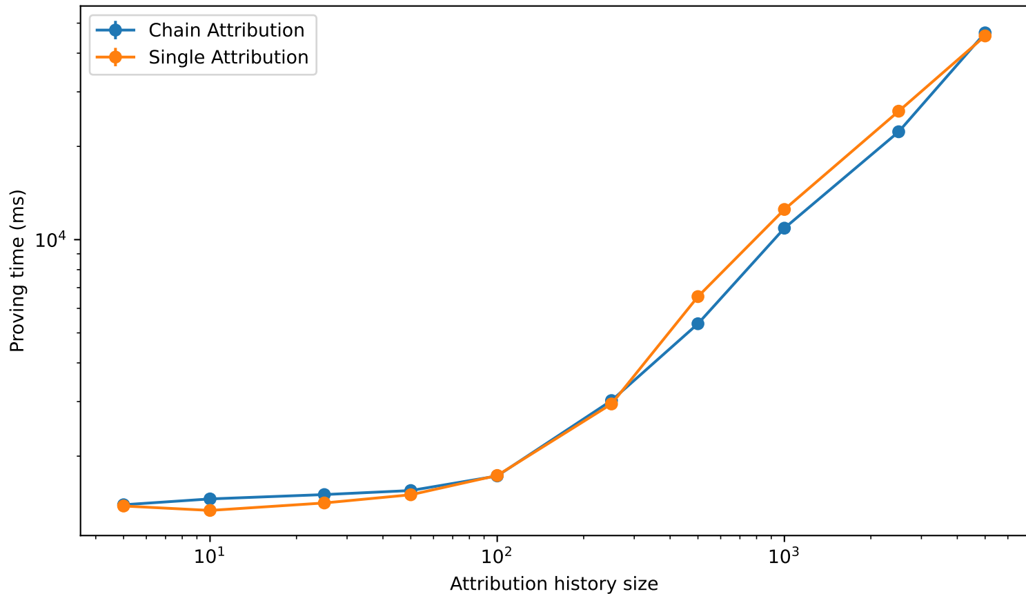
Proving Time for Attribution by Attribution History Size
