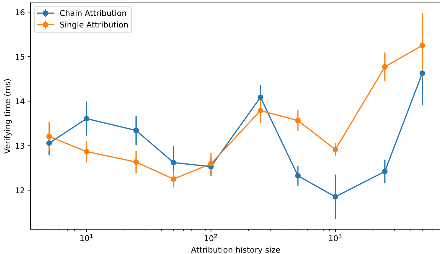
Verifying Time for Attribution by Attribution History Size
