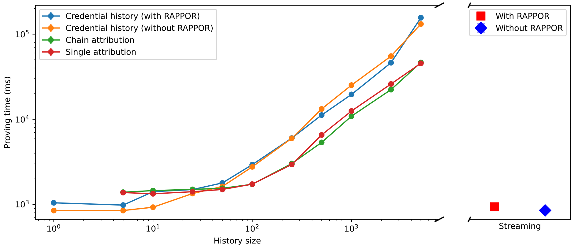
Proving Time for all Circuit Variants Credential histories with and without RAPPOR, attribution histories, streaming algorithm
