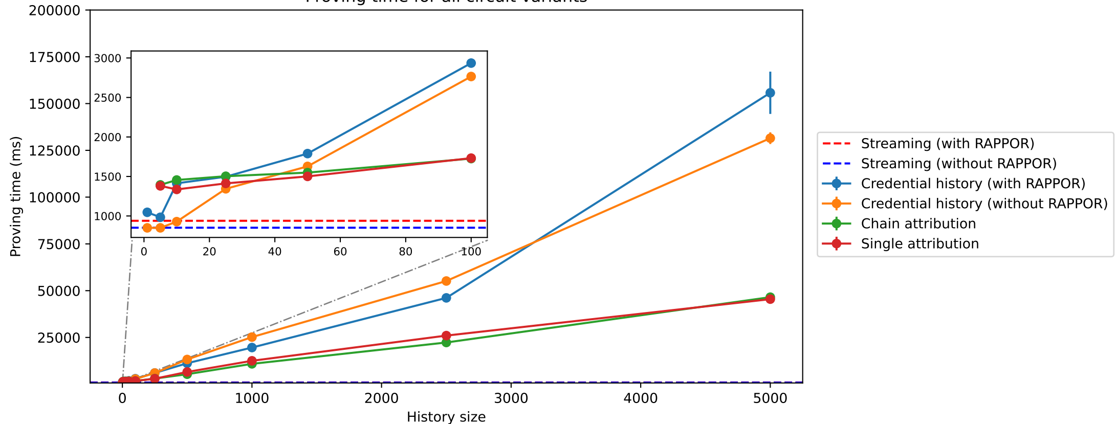
Proving time for all circuit variants
