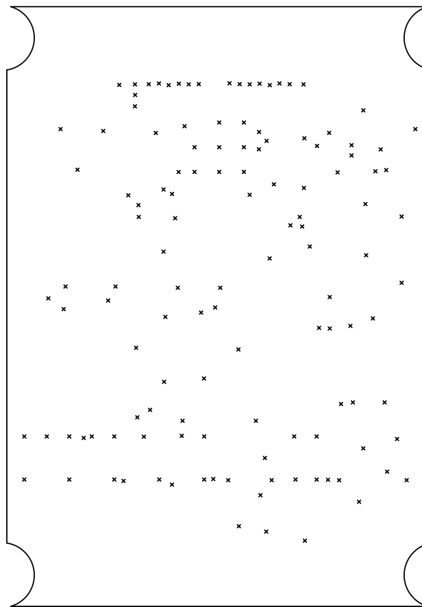
Drill Map: x 0.250mm / 0.0098" (126 holes)
