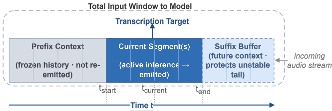
Fig. 2. Schematic of the context-aware ASR sliding-window mechanism.
