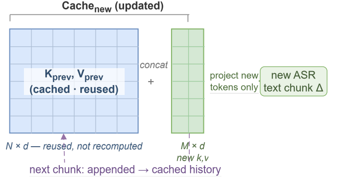
Fig. 3. Schematic of the LLM KV cache incremental update mechanism.
