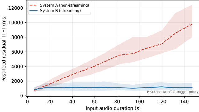
Fig. 4. Descriptive legacy post-feed residual TTFT over independently formed equal-frequency duration bins. System A uses 1,133 error-free archived records; System B uses 1,132 after one streaming runtime error was omitted. Lines show bin means and shaded regions show observed P5–P95 ranges, not confidence intervals; this is not a paired-bin analysis.
