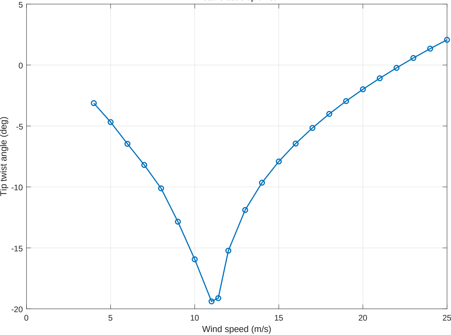
Total elastic tip twist
