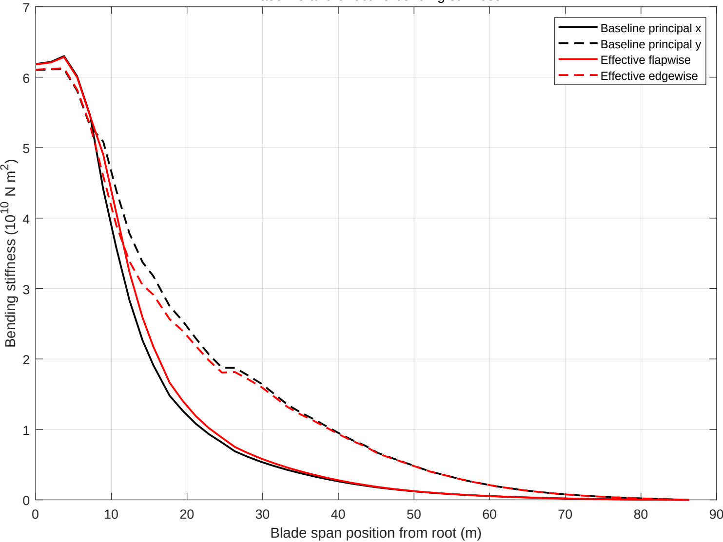
Baseline and effective bending stiffness
