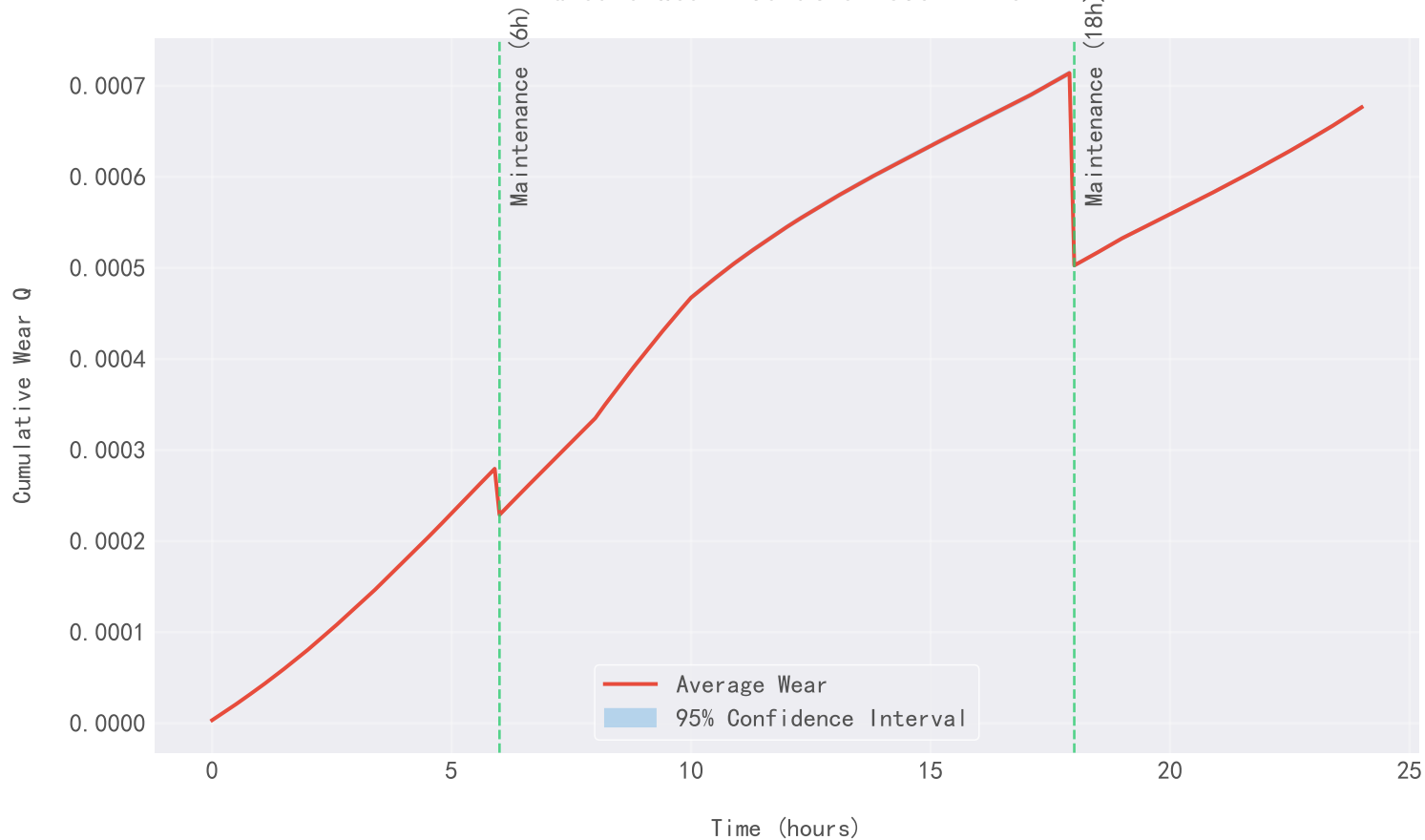
Ground Wear Evolution Over Time
