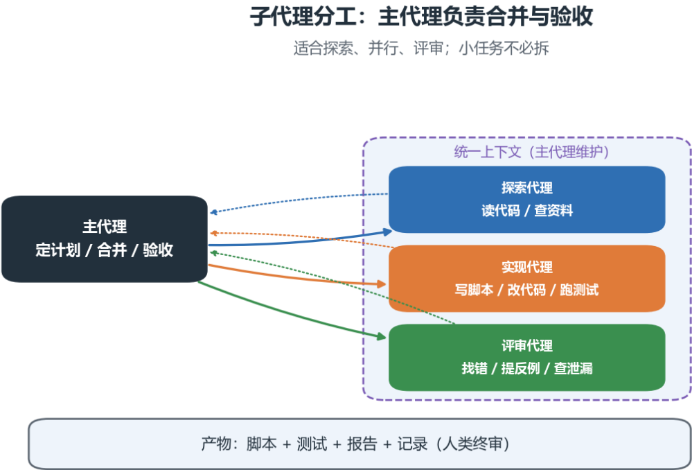
Figure 57: 子代理分工
