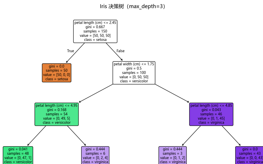
Figure 2: Iris 决策树
