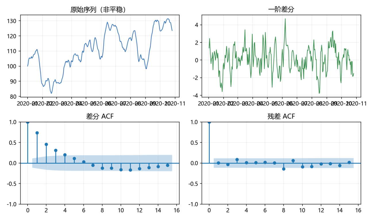
Figure 40: ARIMA 选阶与残差诊断图
