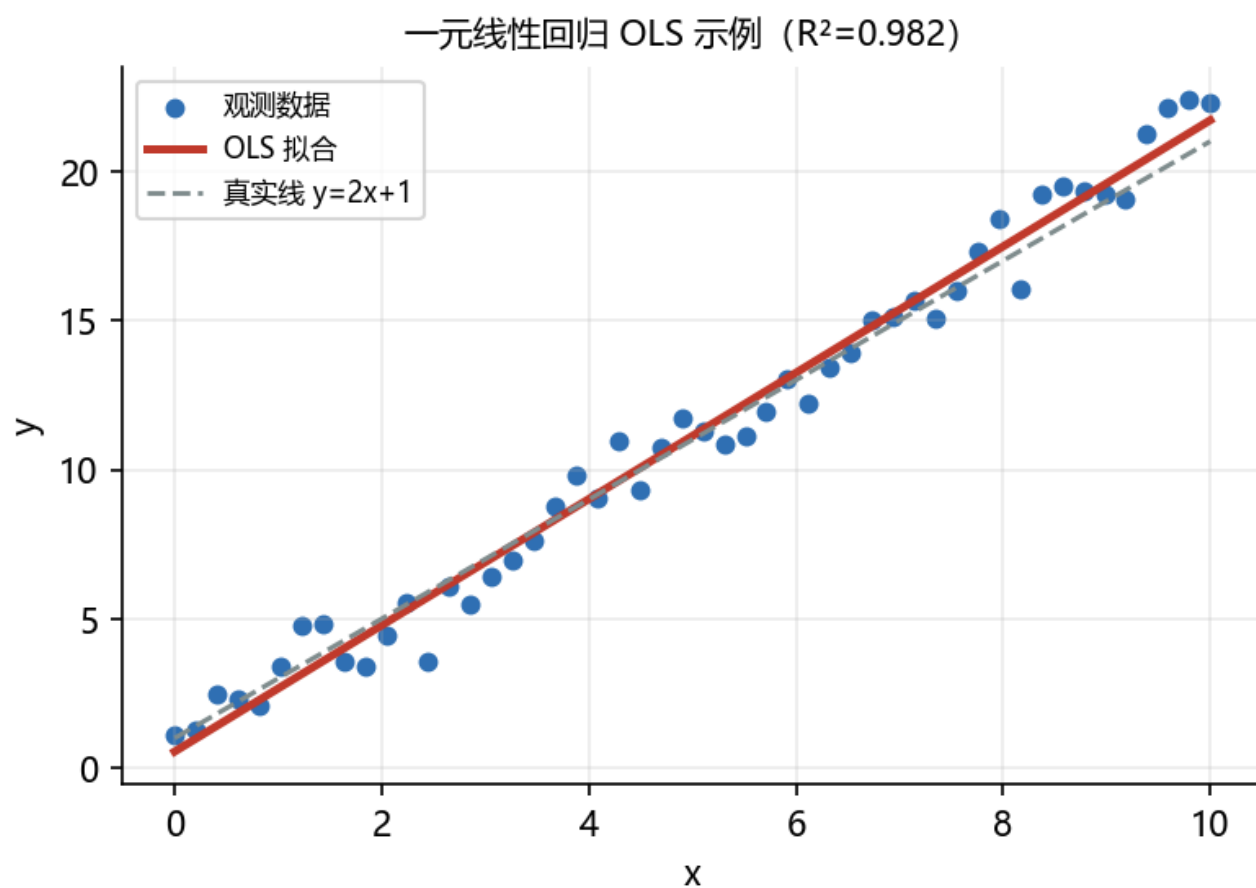
Figure 35: OLS 拟合示意
