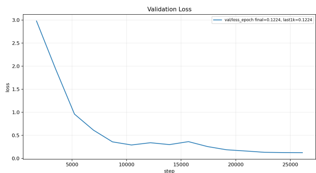
(a) Factored 96/96 val loss
