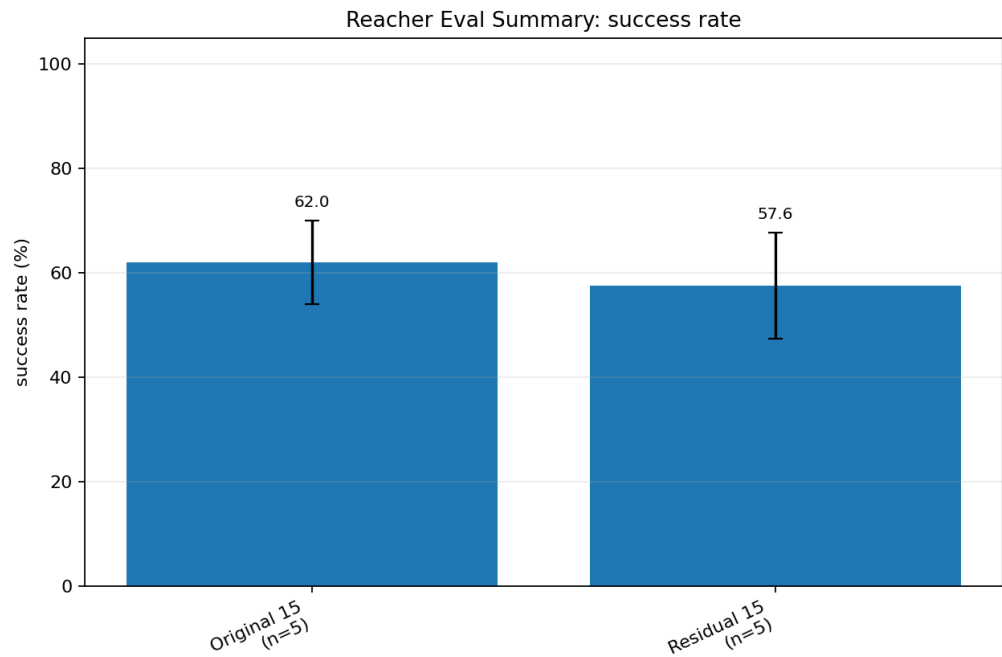
图 4: Reacher success rate mean \pm std
