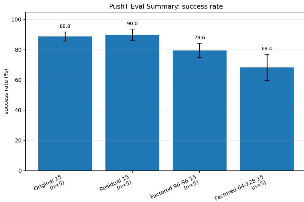
图 1: PushT success rate mean \pm std
