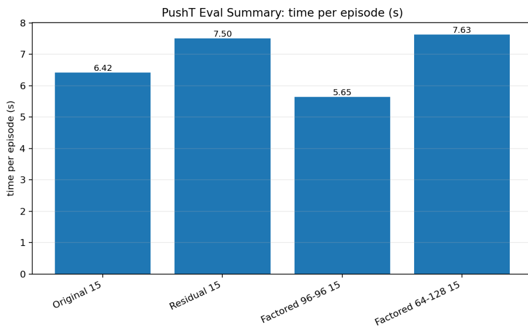
图 3: PushT time per episode
