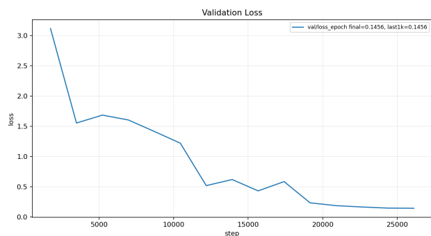
(b) Factored 64/128 val loss
