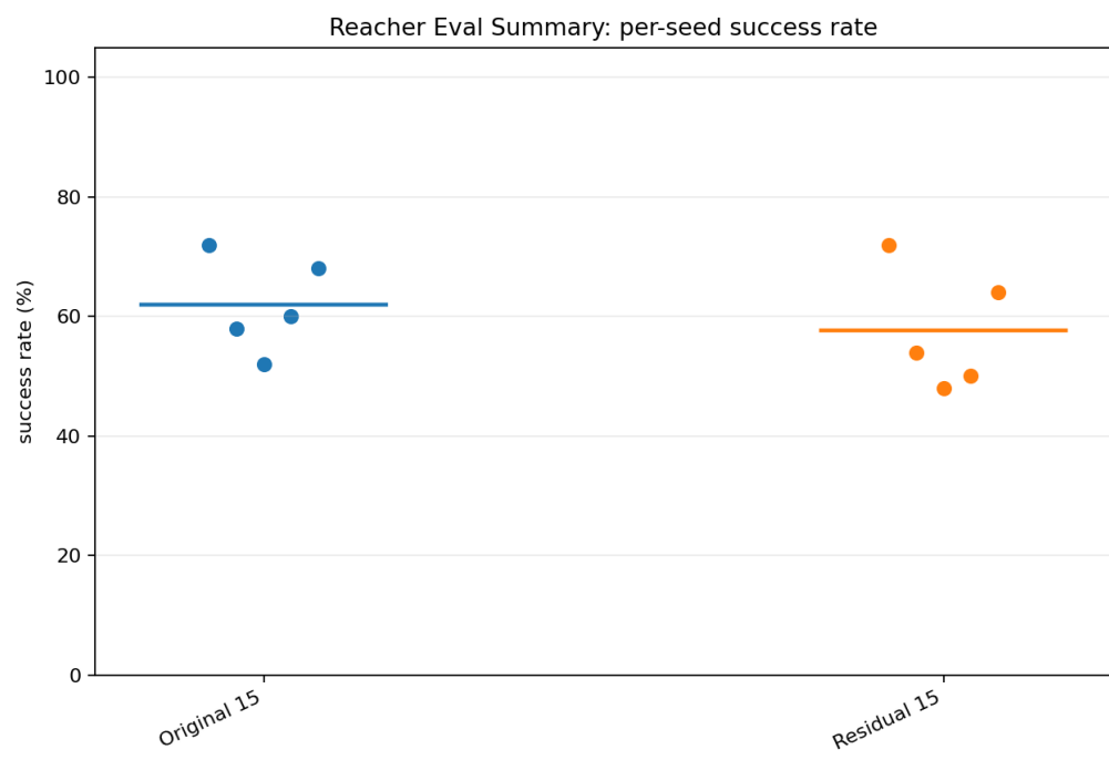
图 5: Reacher per-seed success rate
