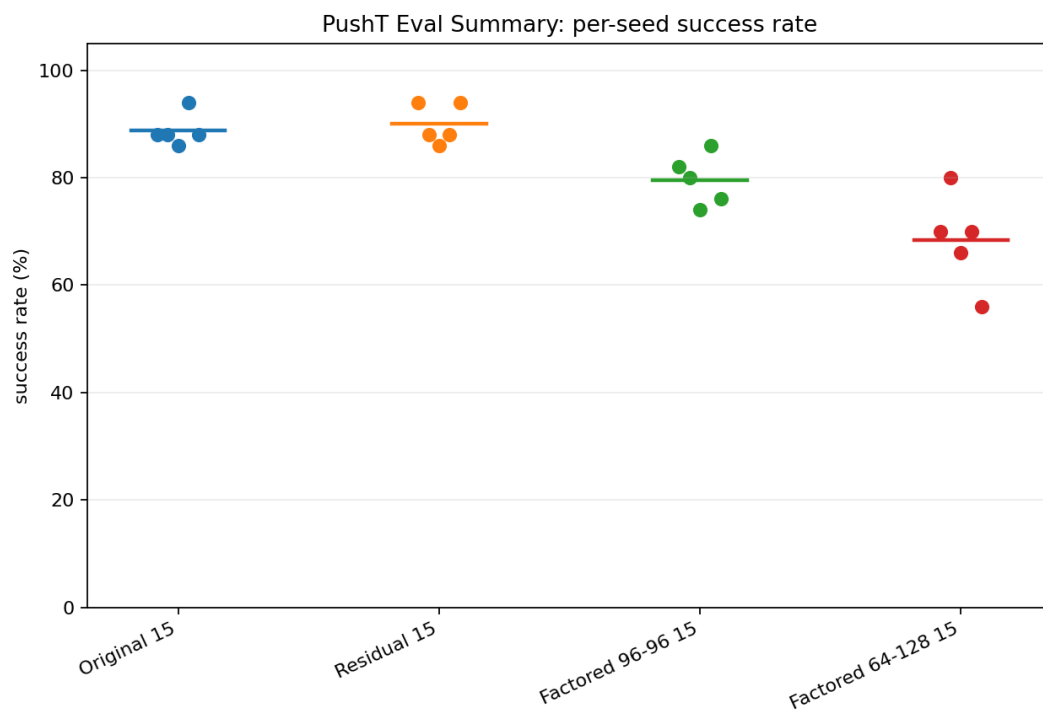
图 2: PushT per-seed success rate
