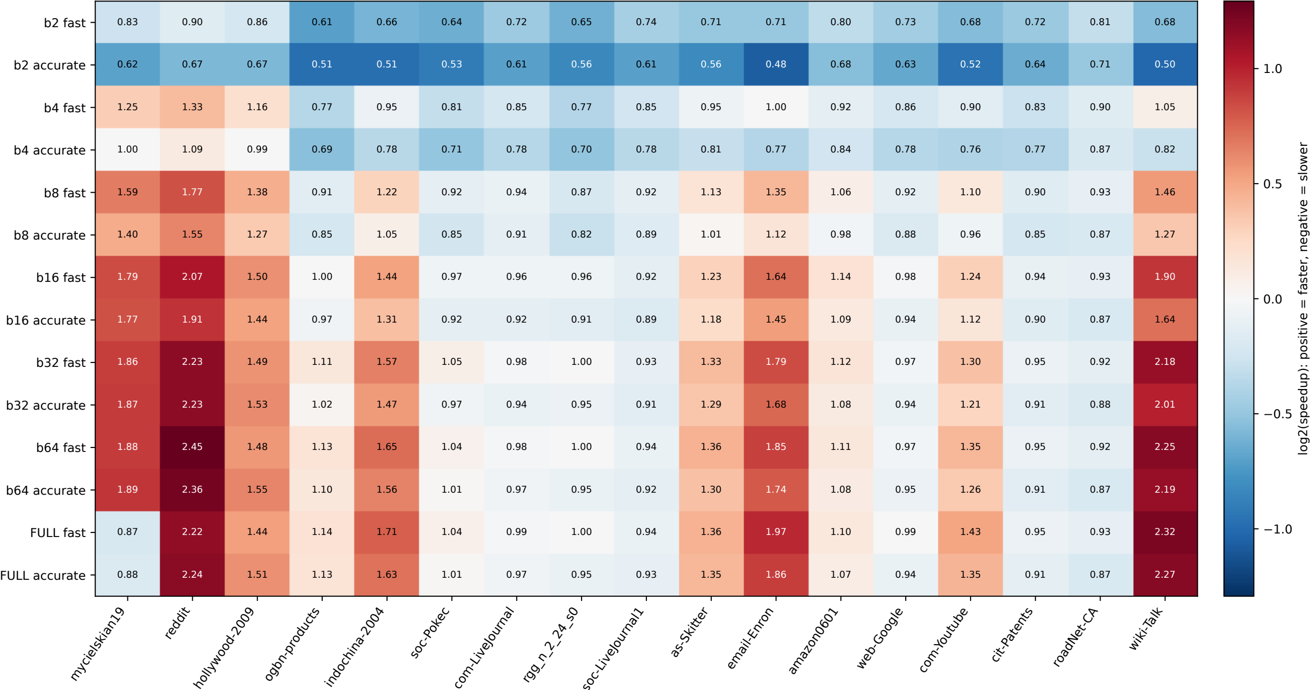
Graphs ordered by average degree (highest to lowest)
