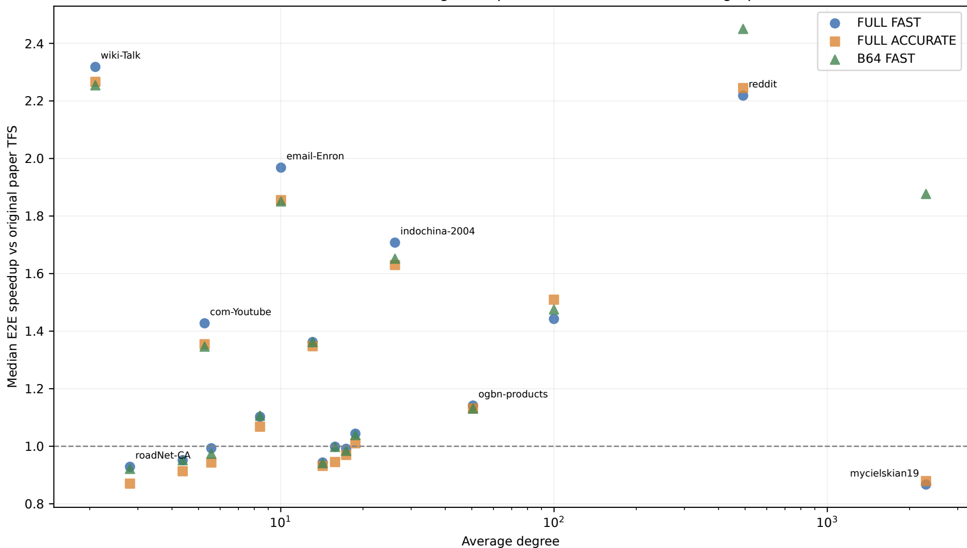
Interleaved execution: degree-dependent crossover, all 17 real graphs
