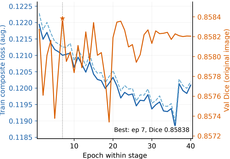
Mean-Hinge ( \lambda = 1 ) DONE 40/40
